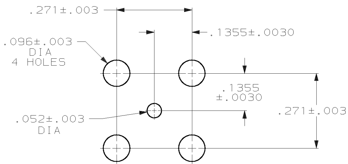
PCB CONFIGURATION
